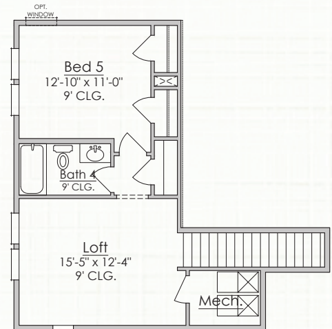
2nd Floor Plan 541 Sq.Ft.
