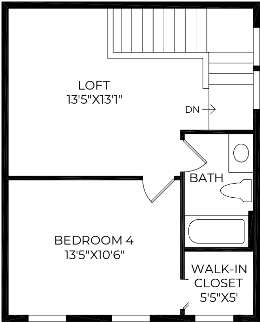
SECOND FLOOR 9' CEILING HEIGHT
