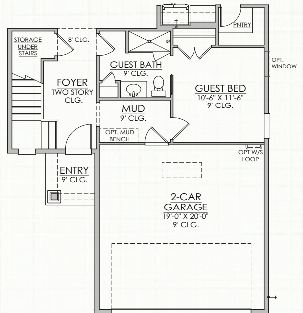
Optional Guest Bed & Bath In Lieu of Tandem Garage & Powder Bath
