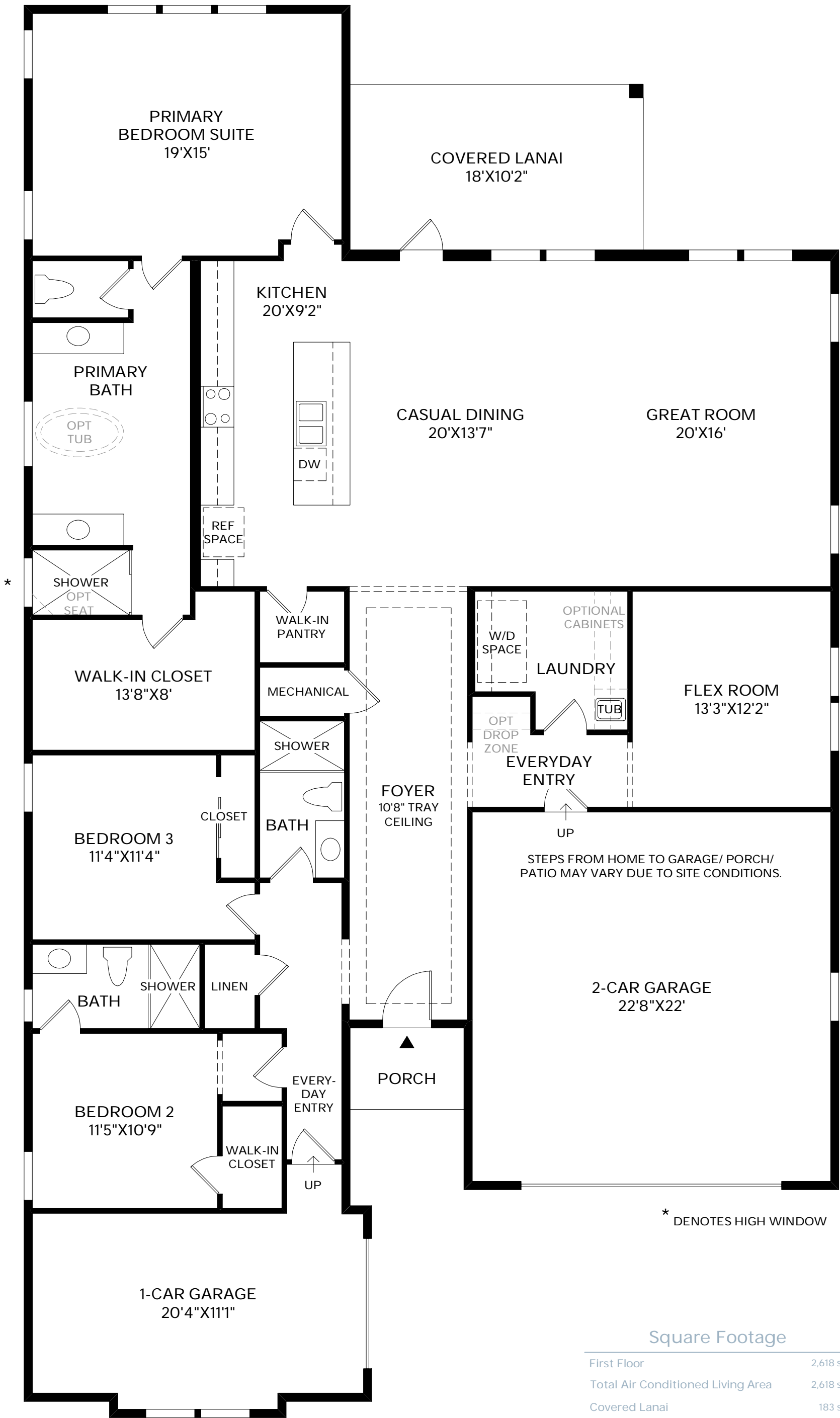
FLOOR PLAN 10' CEILING HEIGHT
